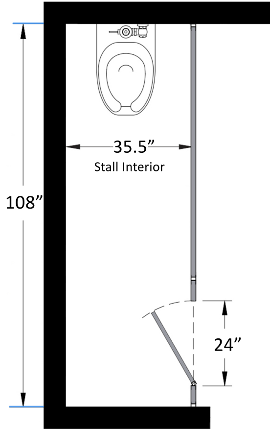
Bathroom Partitions - 1 Stall Alcove Left Hand SKU: ALIC1L Standard Dimensions
